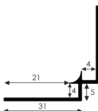
134220 Binnenhoekprofiel 4/4100 anod (+T) Internal corner 4/4100 anod (+T) Inneneckprofil 4/4100 elox (+T)
